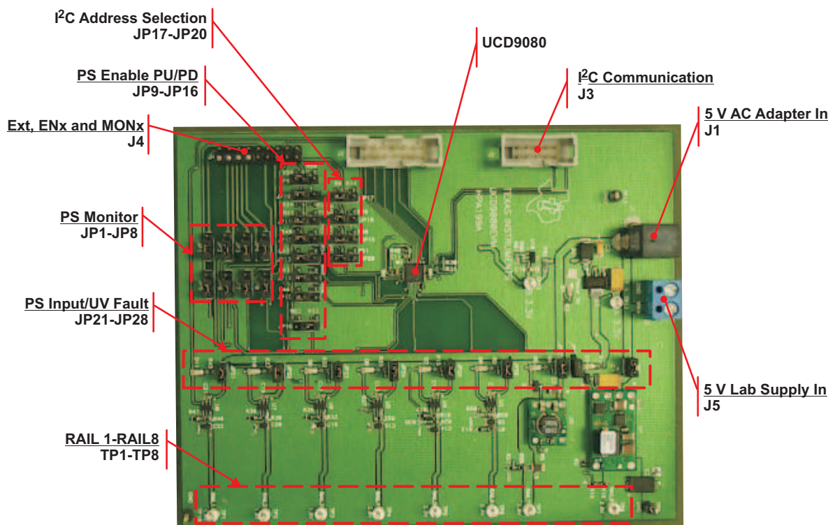
Figure 1. UCD9080EVM
